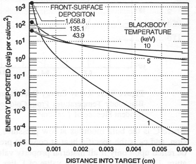
Figure 7.10. ANISN Deposition Profile for Tantalum at Blackbody Temperatures of 1, 5, and 10 keV (Incident Fluence = 1 cal/cm 2 ).
